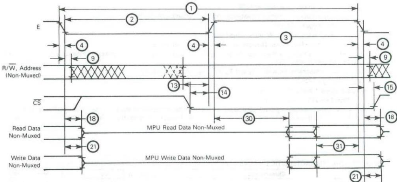
FIGURE 1 — BUS TIMING
