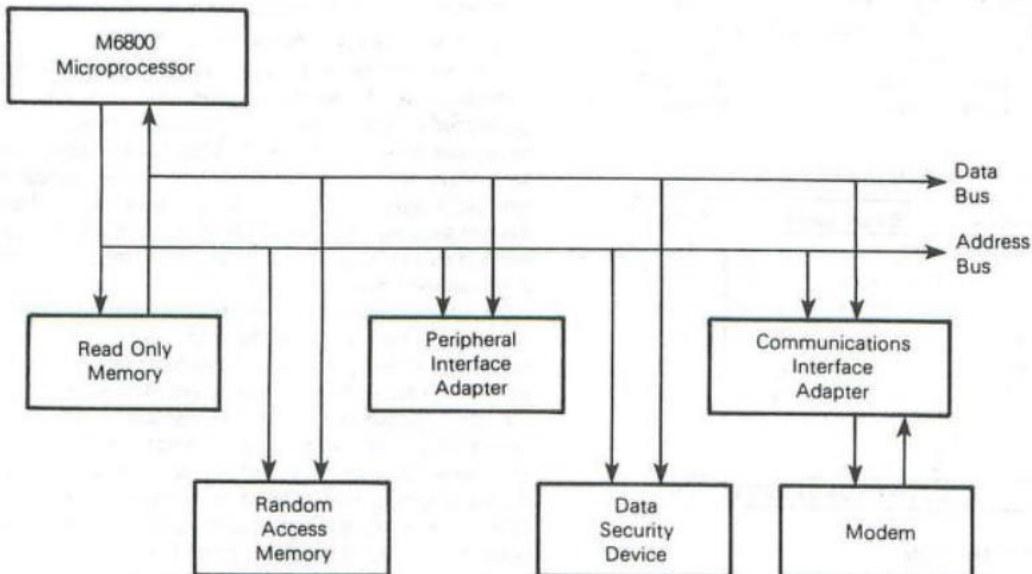
FIGURE 4 — M6800 MICROCOMPUTER FAMILY BLOCK DIAGRAM
