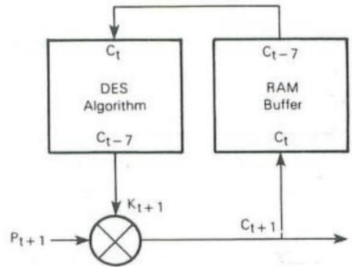
FIGURE 5 — CFB ENCIPHER DATA FLOW (TRANSMITTING)
