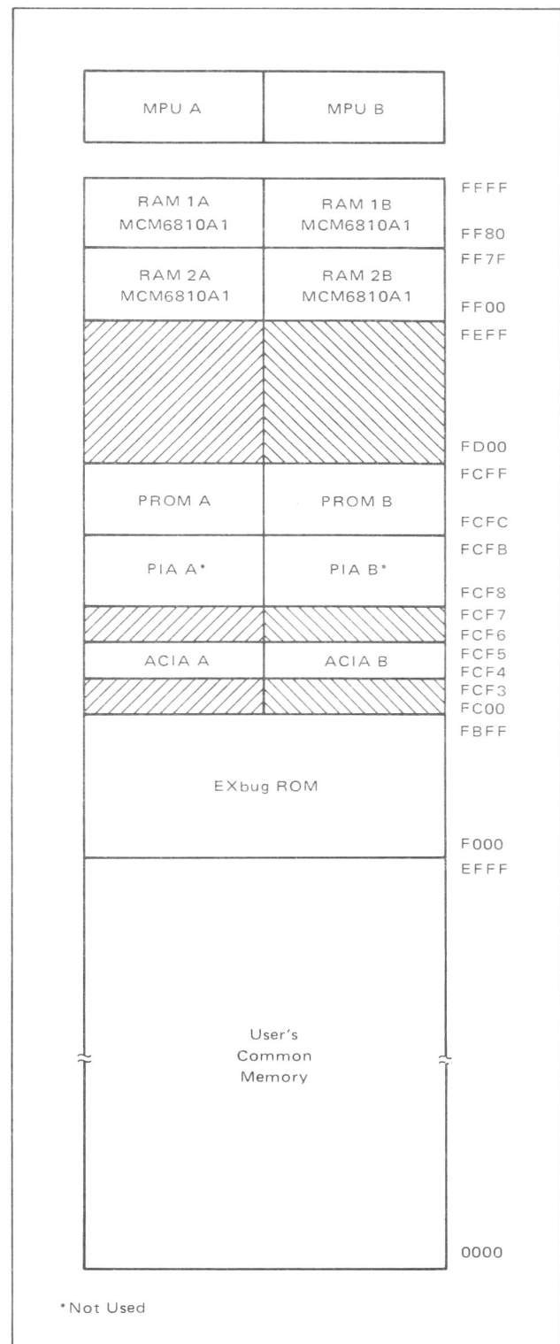
FIGURE 4 — Dual Processor System Memory Map
