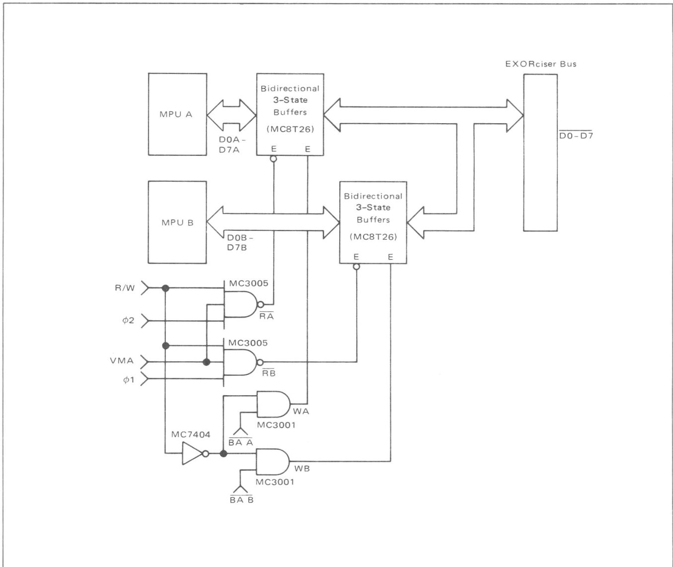
FIGURE 12 — Data Drivers/Receivers
