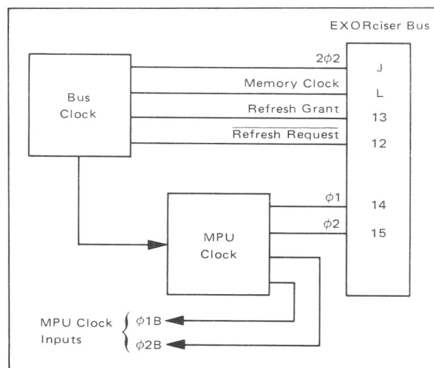
FIGURE 7 — System Clock Block Diagram
