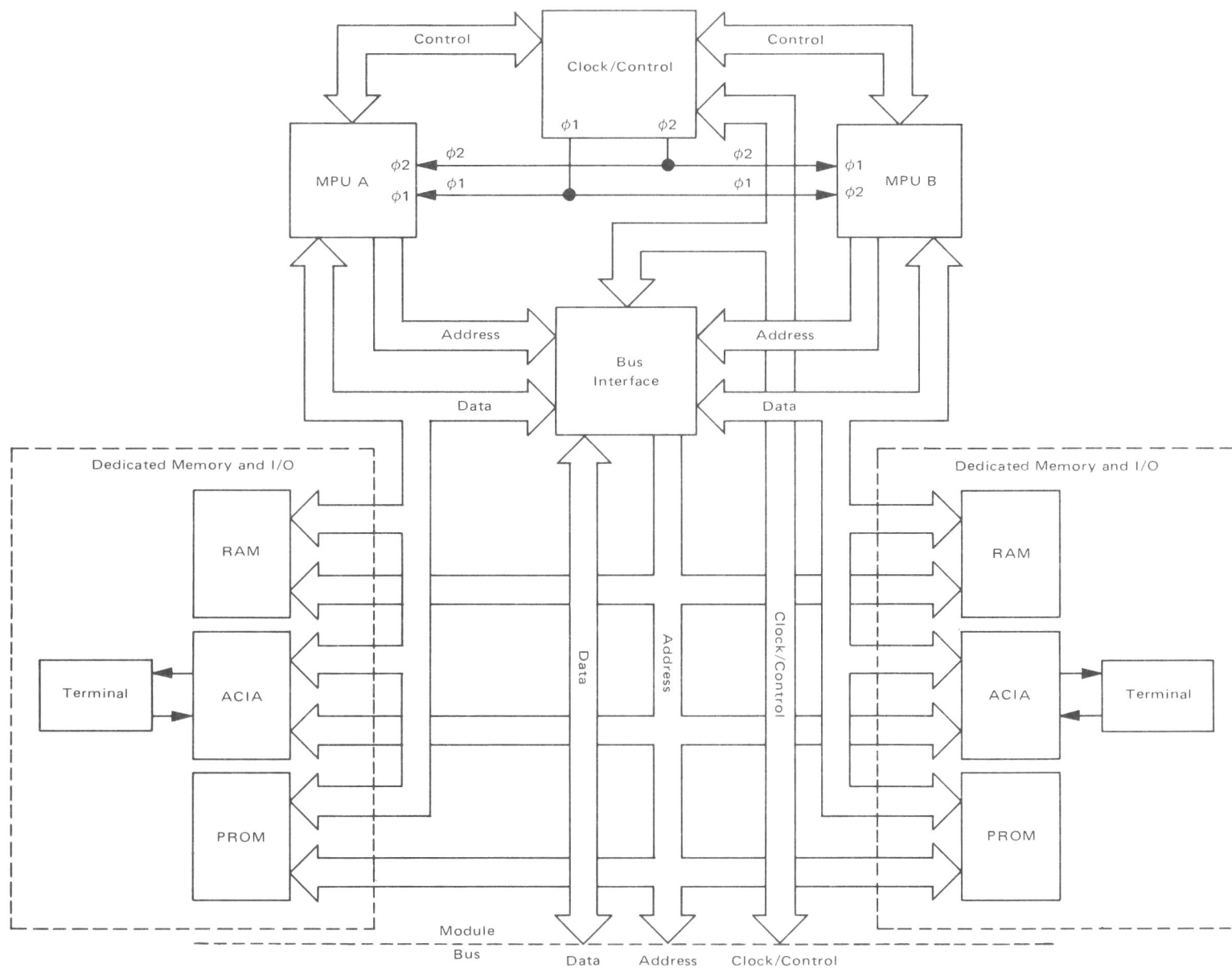
FIGURE 5 – Dual Processor System for Use with EXORciser
