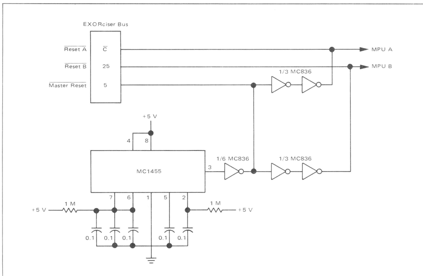
FIGURE 6 — System Reset
