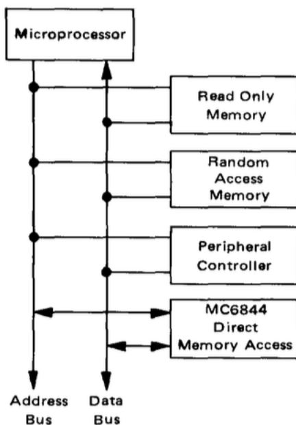
FIGURE 1 — M6800 MICROCOMPUTER FAMILY BLOCK DIAGRAM
