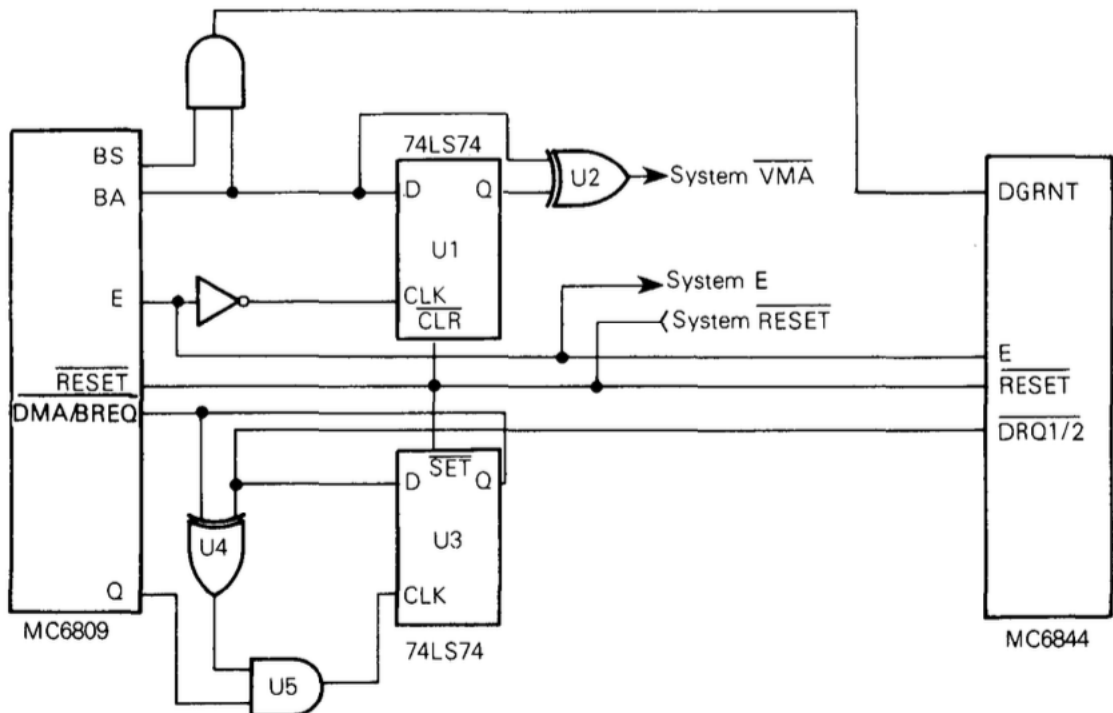
FIGURE 13 — MC6844/MC6809 INTERFACE
