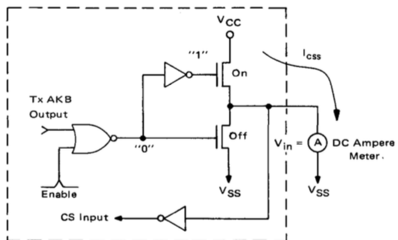
FIGURE 8 — CS/Tx AKB SOURCE CURRENT TEST CIRCUIT
