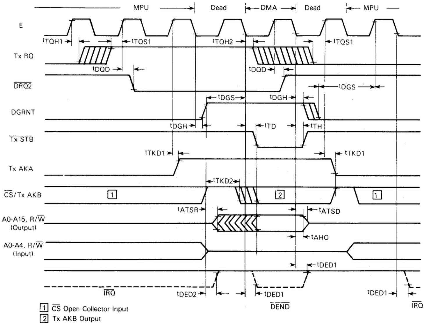
FIGURE 5 — MODE 2 TIMING (HALT STEAL MODE)
