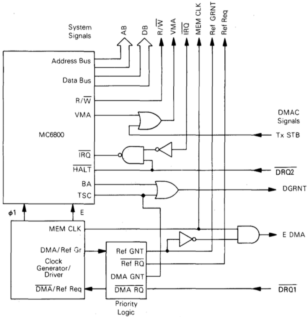
FIGURE 12 — MC6800/MC6844 INTERFACE
