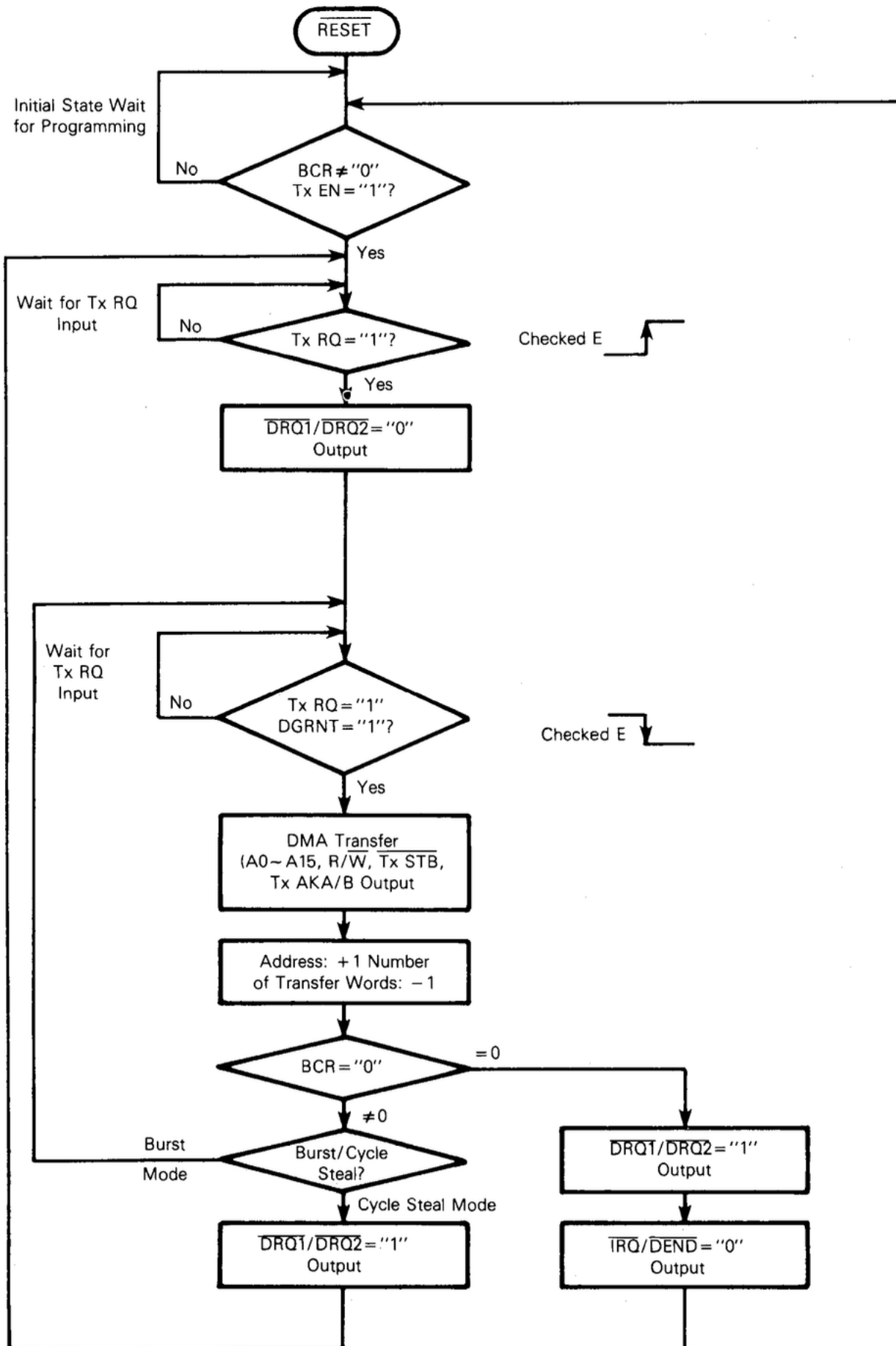
FIGURE 9 — FLOWCHART OF DMAC OPERATION
