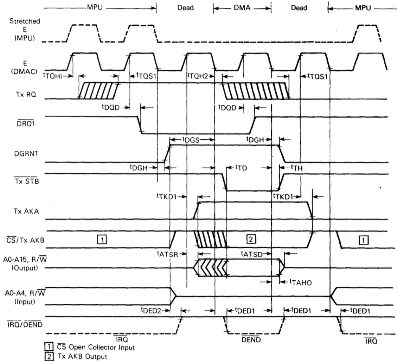
FIGURE 4 — MODE 1 TIMING (TSC STEAL MODE)
