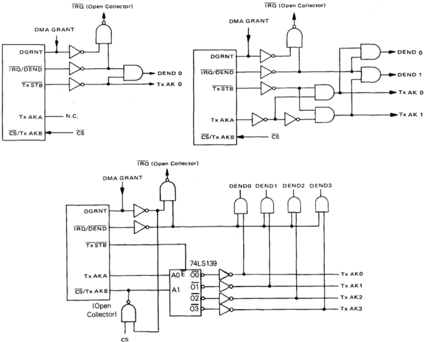
FIGURE 10 — \overline{\text{IRQ}} , DEND, Tx AK GENERATION
