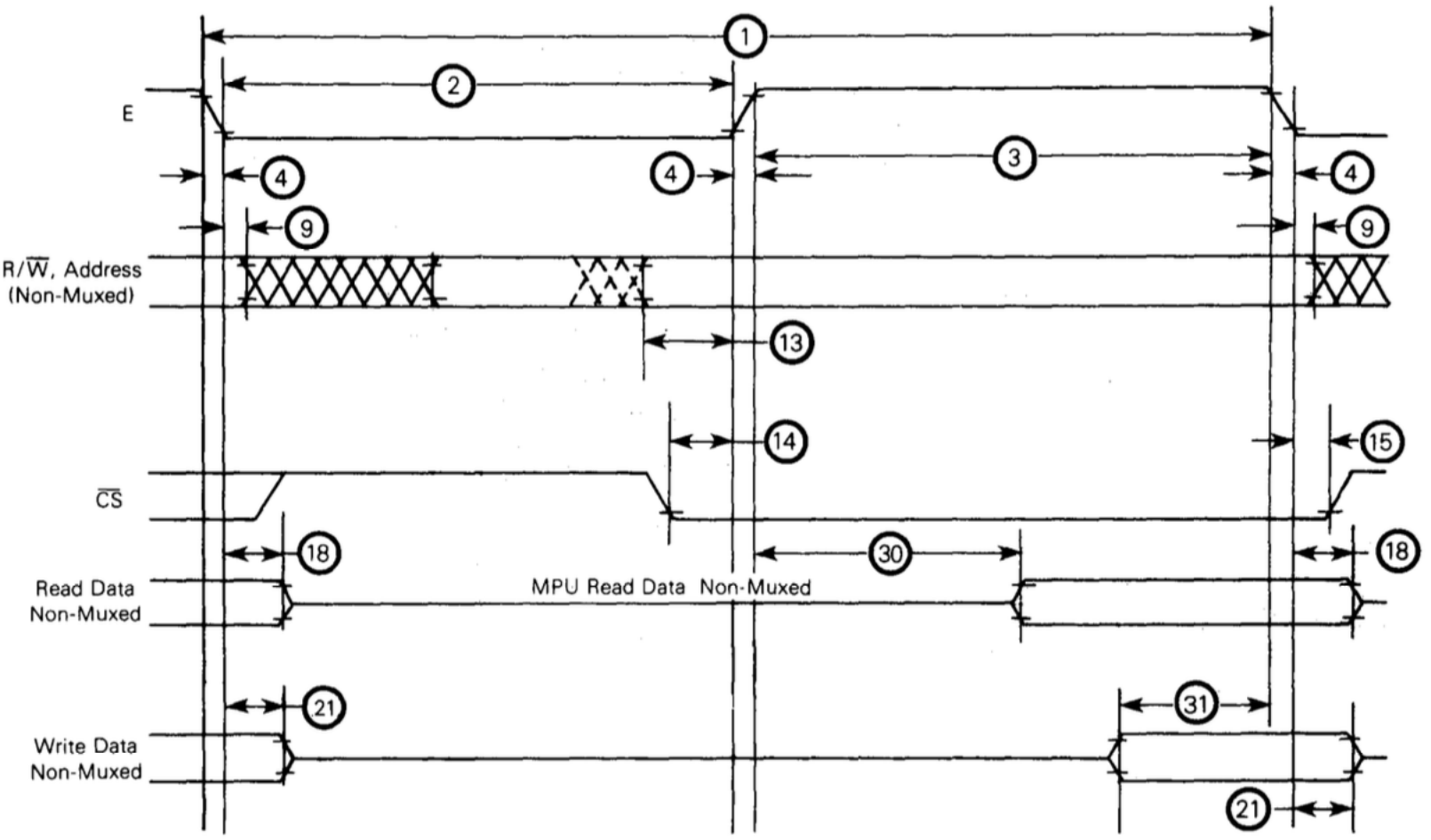
FIGURE 3 — MPU MODE TIMING
