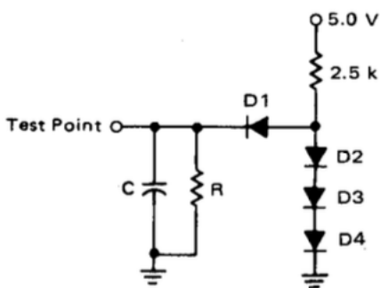
FIGURE 7 — TEST LOADS
