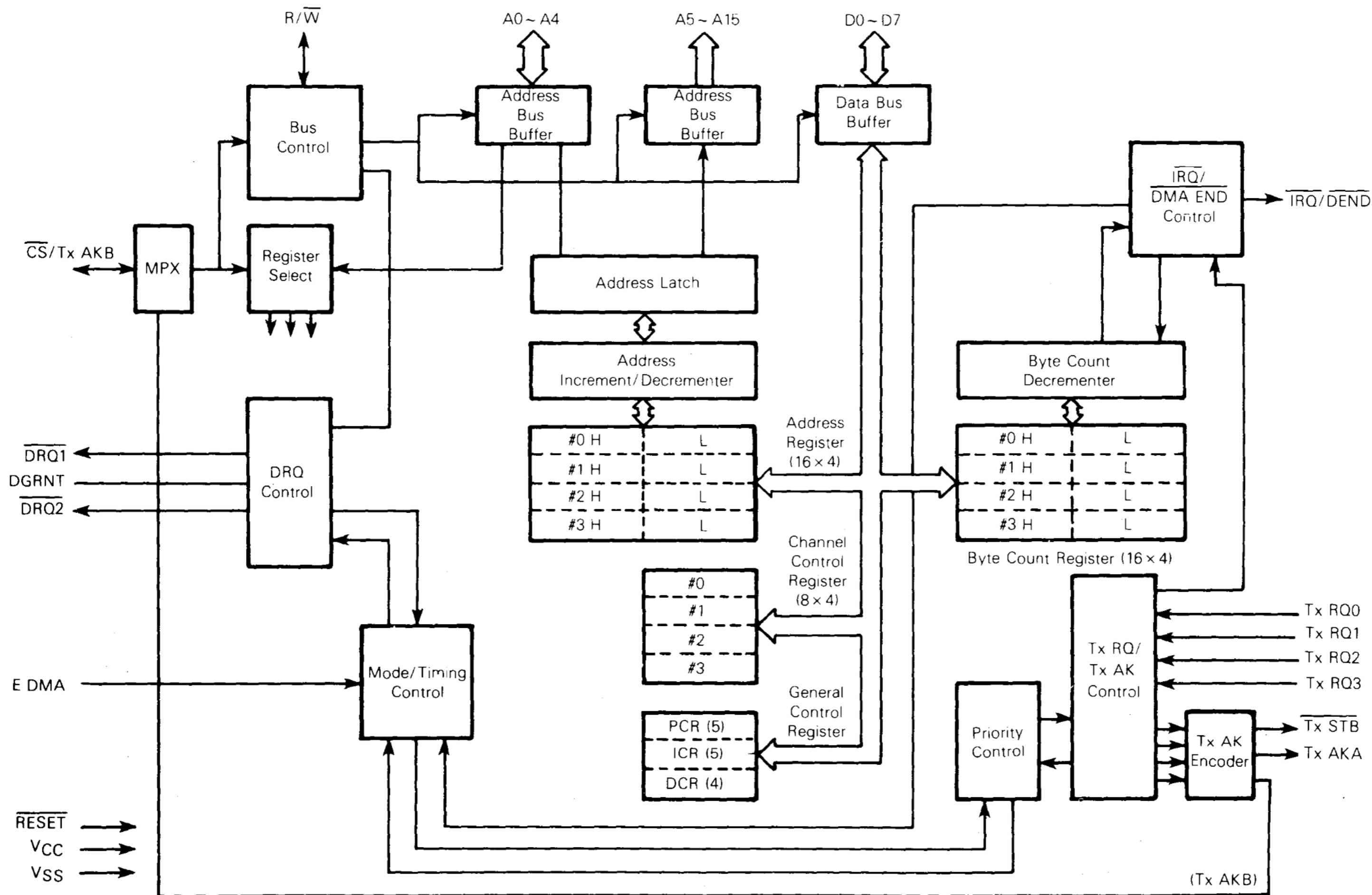
FIGURE 2 — BLOCK DIAGRAM OF DMAC
