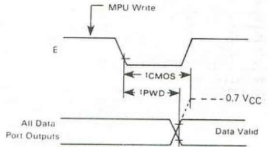
FIGURE 4 — DATA SETUP AND HOLD TIMES (MPU WRITE)
