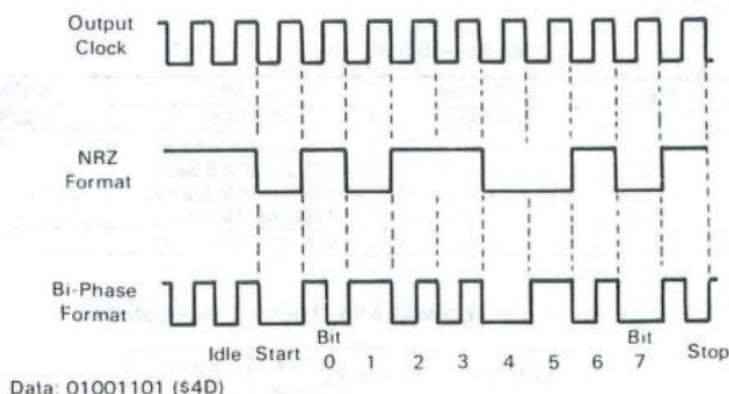
FIGURE 25 — SCI DATA FORMATS
