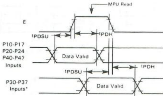
FIGURE 3 — DATA SETUP AND HOLD TIMES (MPU READ)
