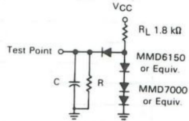
FIGURE 9 — TIMING TEST LOAD PORTS 1, 2, 3, 4
