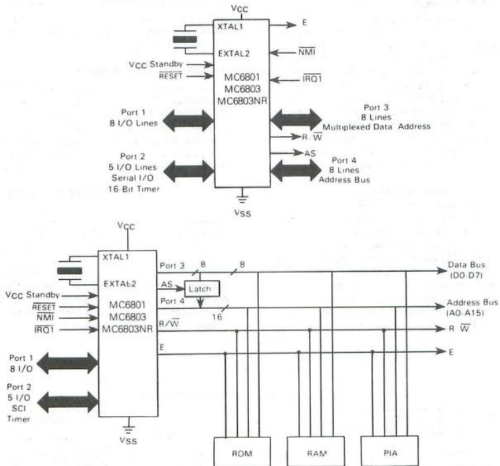
FIGURE 14 — EXPANDED MULTIPLEXED CONFIGURATION
