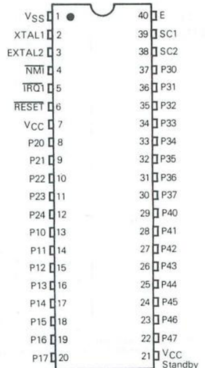
FIGURE 1 — PIN ASSIGNMENT
