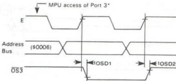
FIGURE 5 — PORT 3 OUTPUT STROBE TIMING (MC6801 SINGLE-CHIP MODE)
