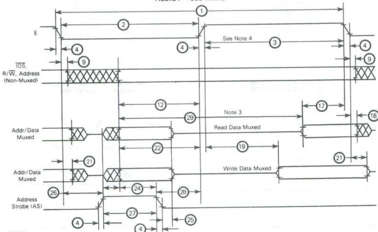
FIGURE 7 — BUS TIMING
