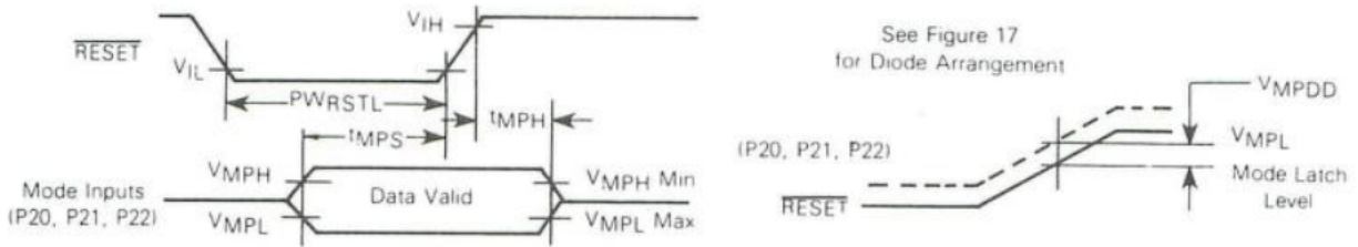
FIGURE 16 — MODE PROGRAMMING TIMING
