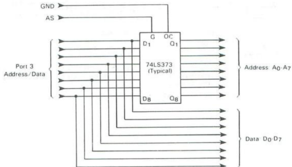
FIGURE 15 — TYPICAL LATCH ARRANGEMENT
