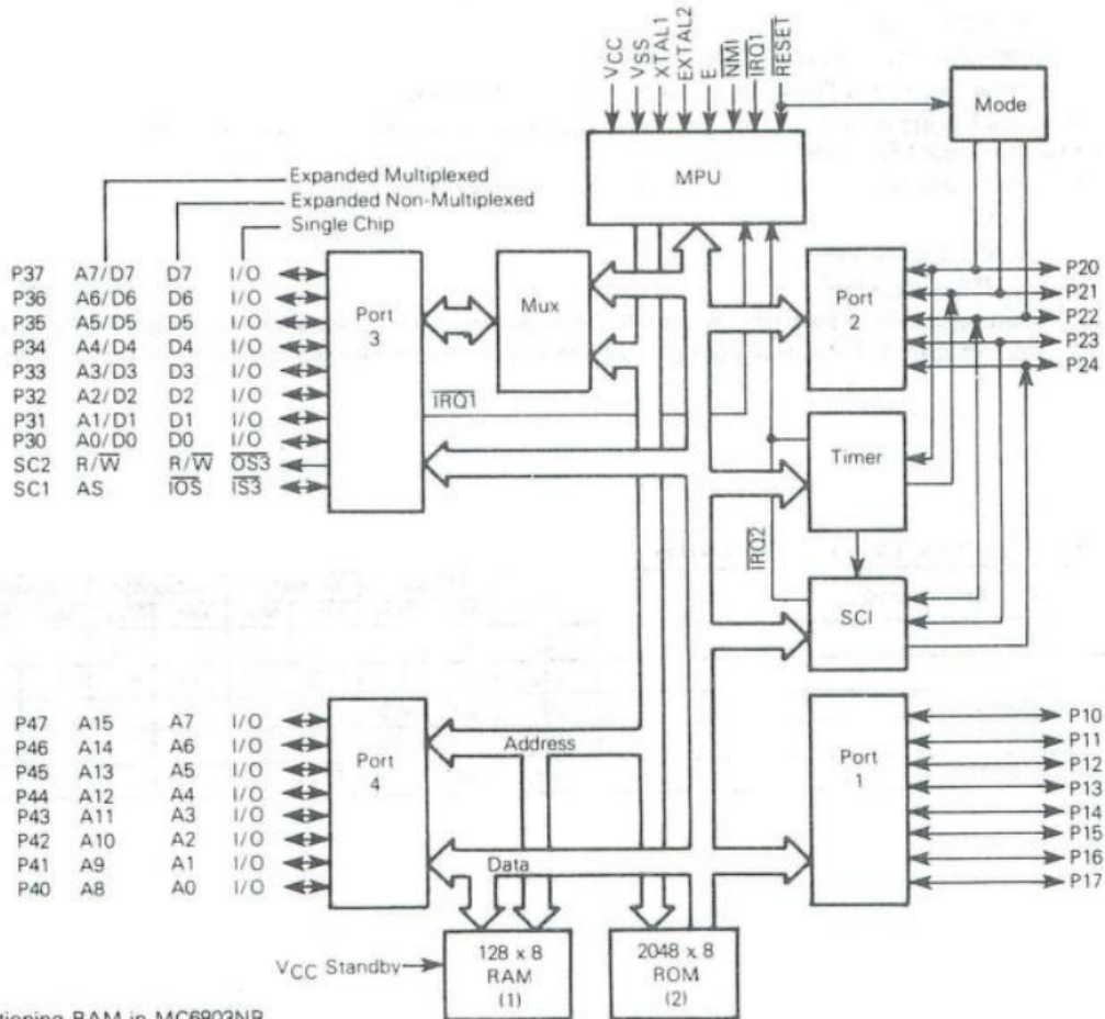
FIGURE 2 — M6801 MICROCOMPUTER FAMILY BLOCK DIAGRAM
