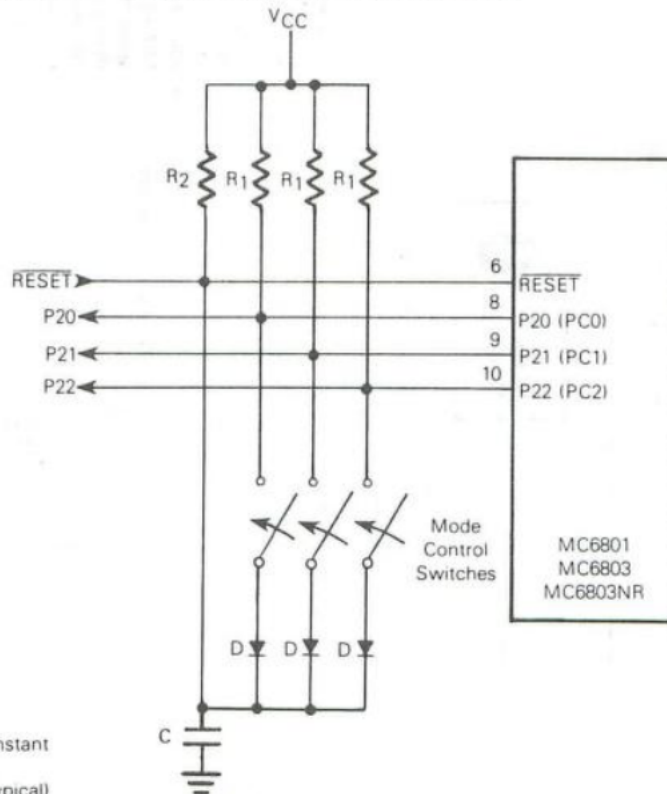
FIGURE 17 — TYPICAL MODE PROGRAMMING CIRCUIT
