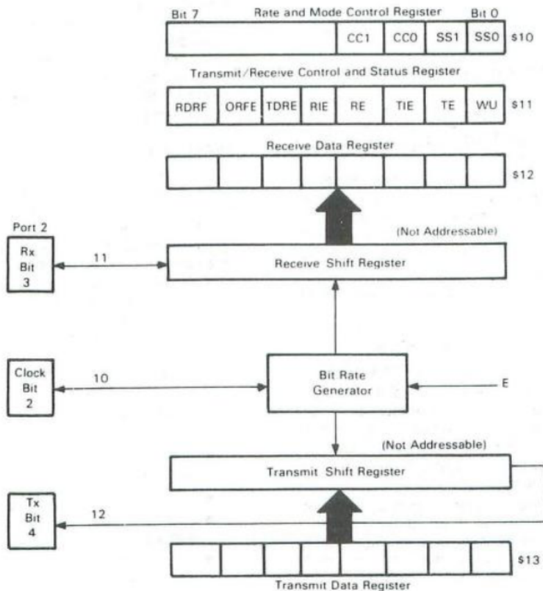
FIGURE 24 — SCI REGISTERS
