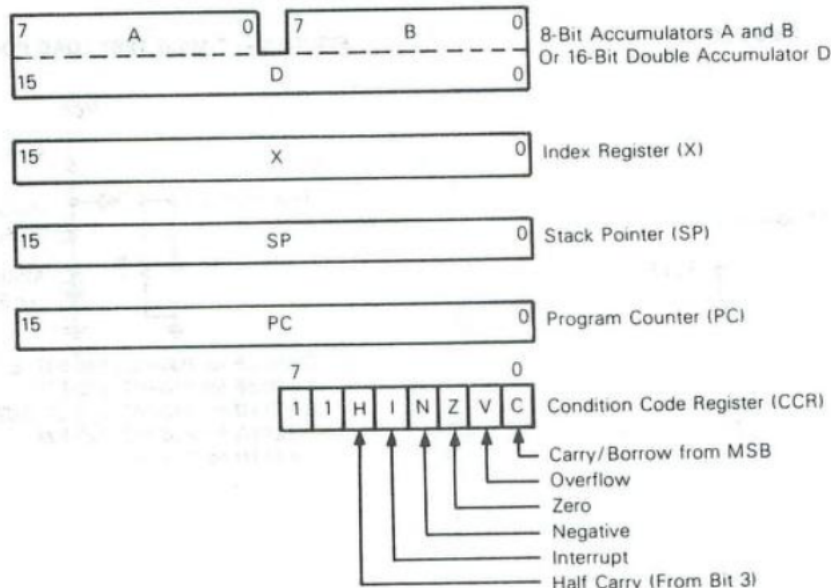
FIGURE 10 — PROGRAMMING MODEL
