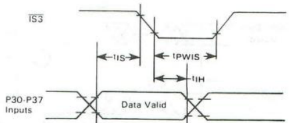
FIGURE 6 — PORT 3 LATCH TIMING (MC6801 SINGLE-CHIP MODE)
