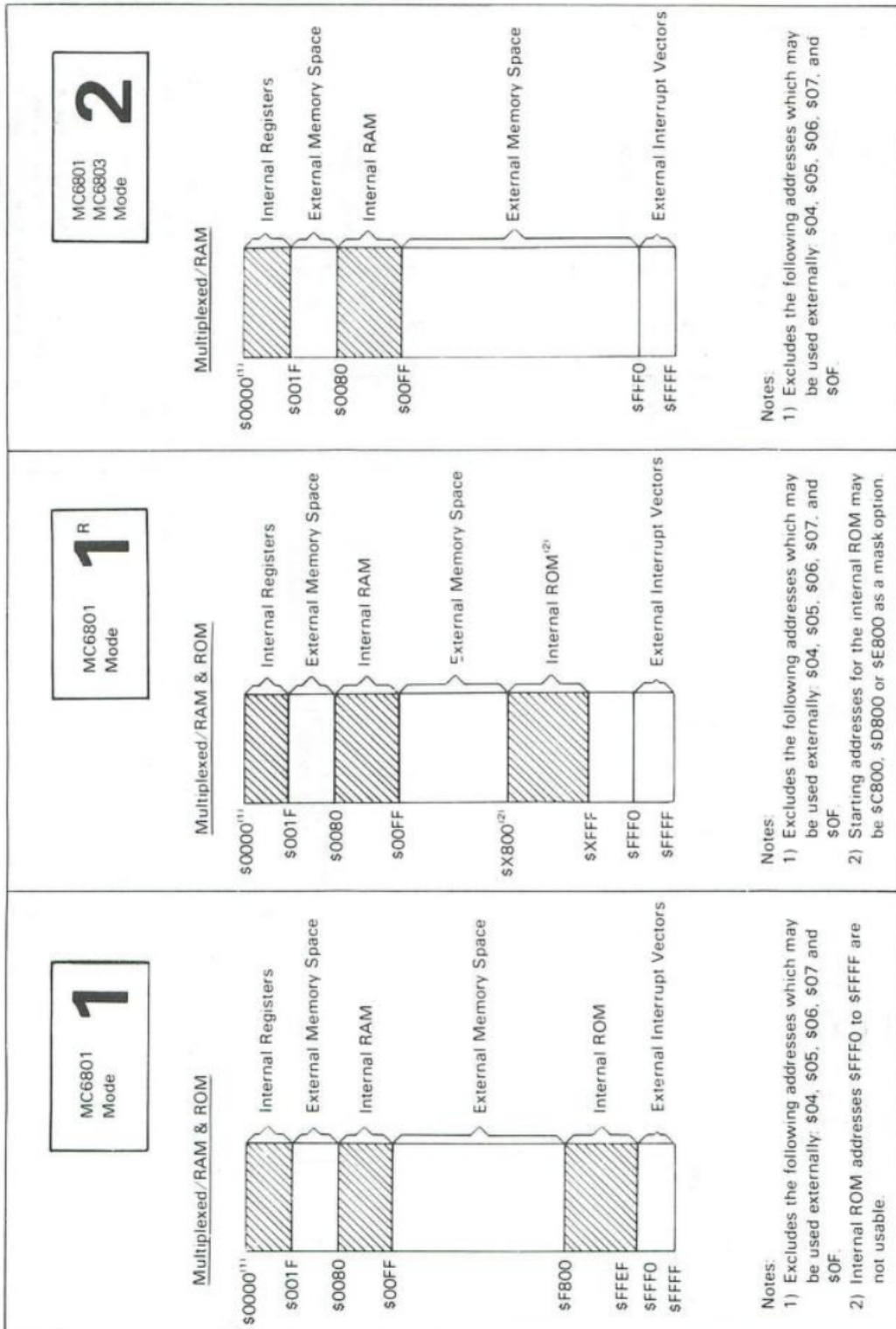
FIGURE 18 — MC6801/03/03NR MEMORY MAPS (CONTINUED)
