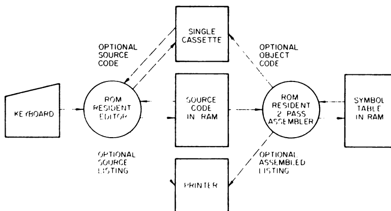
EDITOR/ASSEMBLER BLOCK DIAGRAM
