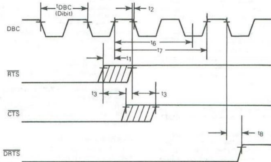
FIGURE 5 — LOSS OF \overline{RTS} TO \overline{DRTS} DELAY
