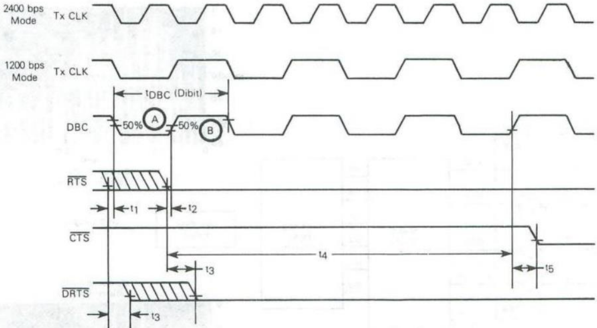
FIGURE 4 — \overline{\text{RTS}} -CTS AND \overline{\text{RTS}} -DRTS DELAYS
