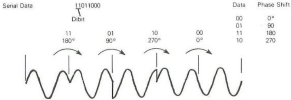
FIGURE 8 — EXAMPLE-CARRIER PHASE SHIFTS FOR OPTION A
