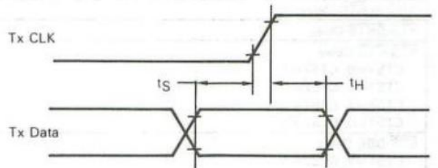
FIGURE 2 — TRANSMIT DATA SETUP AND HOLD TIME
