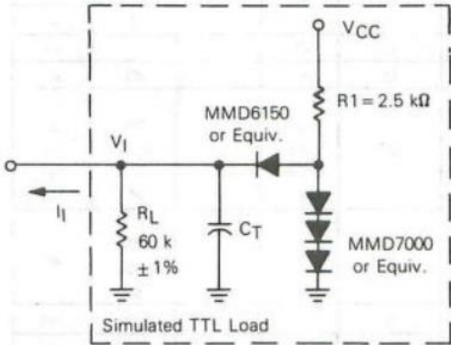
FIGURE 1 — OUTPUT TEST LOAD
