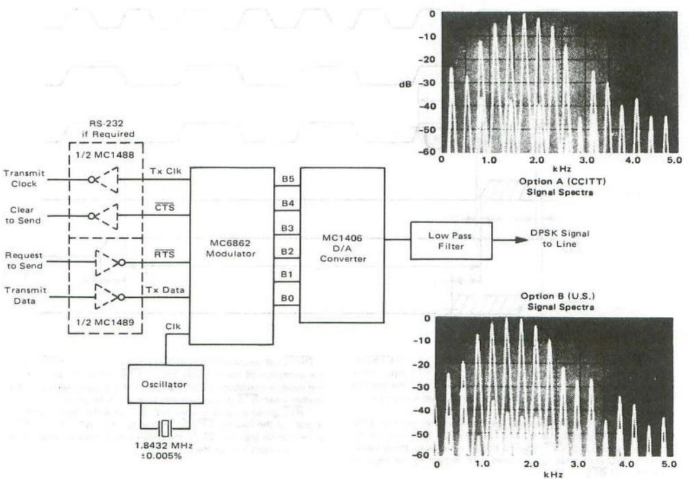
FIGURE 3 — 2400 bps MODULATOR INTERFACE
