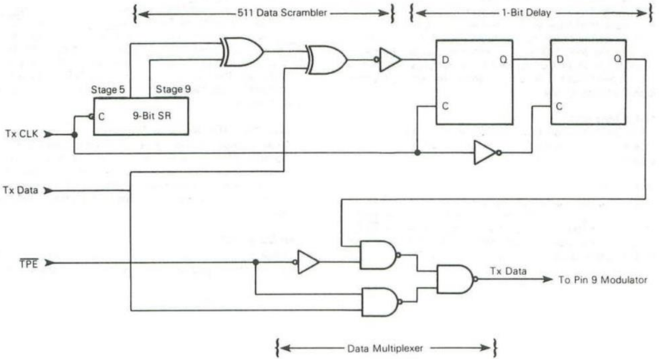
FIGURE 7 — MODULATOR CCITT 511 DATA SCRAMBLER
